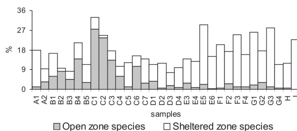
Fig. 4 - Percent values of foraminifers characteristic of sheltered and open zone.
