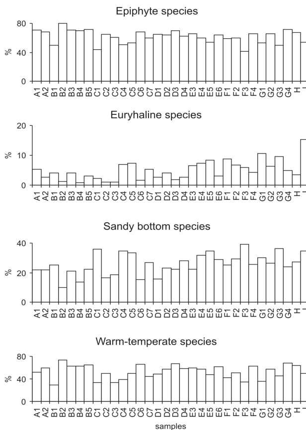
Fig. 3 - Percent values of foraminifer ecological groups.
