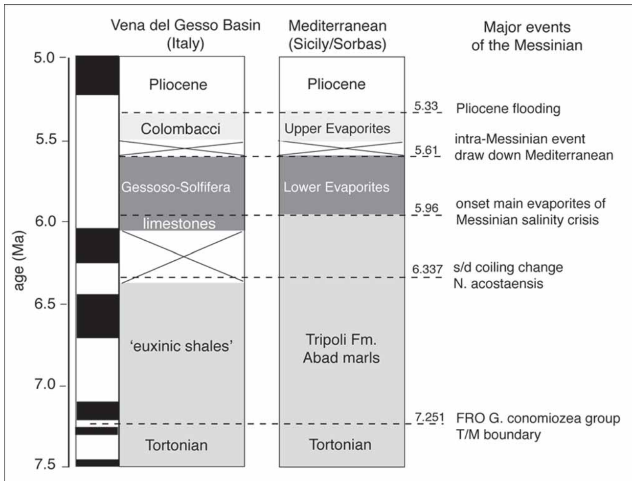
Fig. 1 - The chronology of Messinian events (modified from Krijgsman et al., 1999b).
