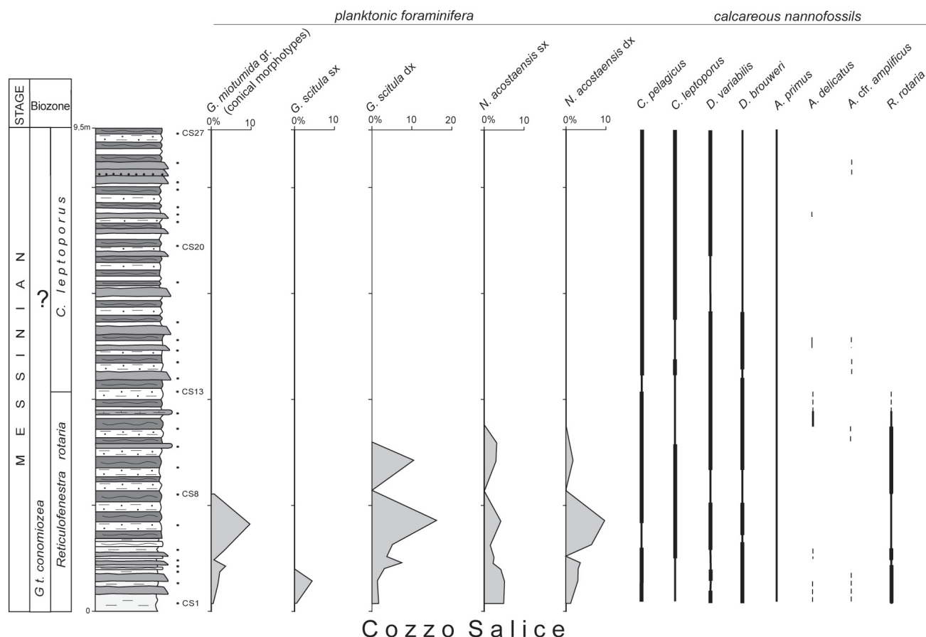
Fig. 8 - Quantitative (planktonic foraminifera) and semiquantitative (calcareous nannofossils) distributions of selected taxa in the Cozzo Salice section. Distribution line thickness of calcareous nannofossils qualitatively reflect the relative abundance of the taxa: rare, common, and very common.
