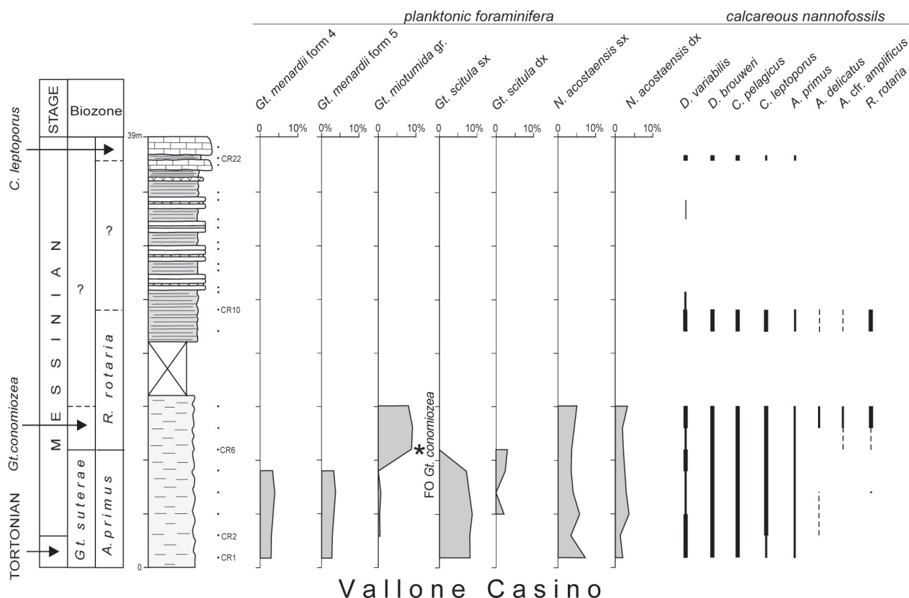
Fig. 9 - Quantitative (planktonic foraminifera) and semiquantitative (calcareous nannofossils) distributions of selected taxa in the Vallone Casino section. Distribution line thickness of calcareous nannofossils qualitatively reflect the relative abundance of the taxa: rare, common, and very common.
