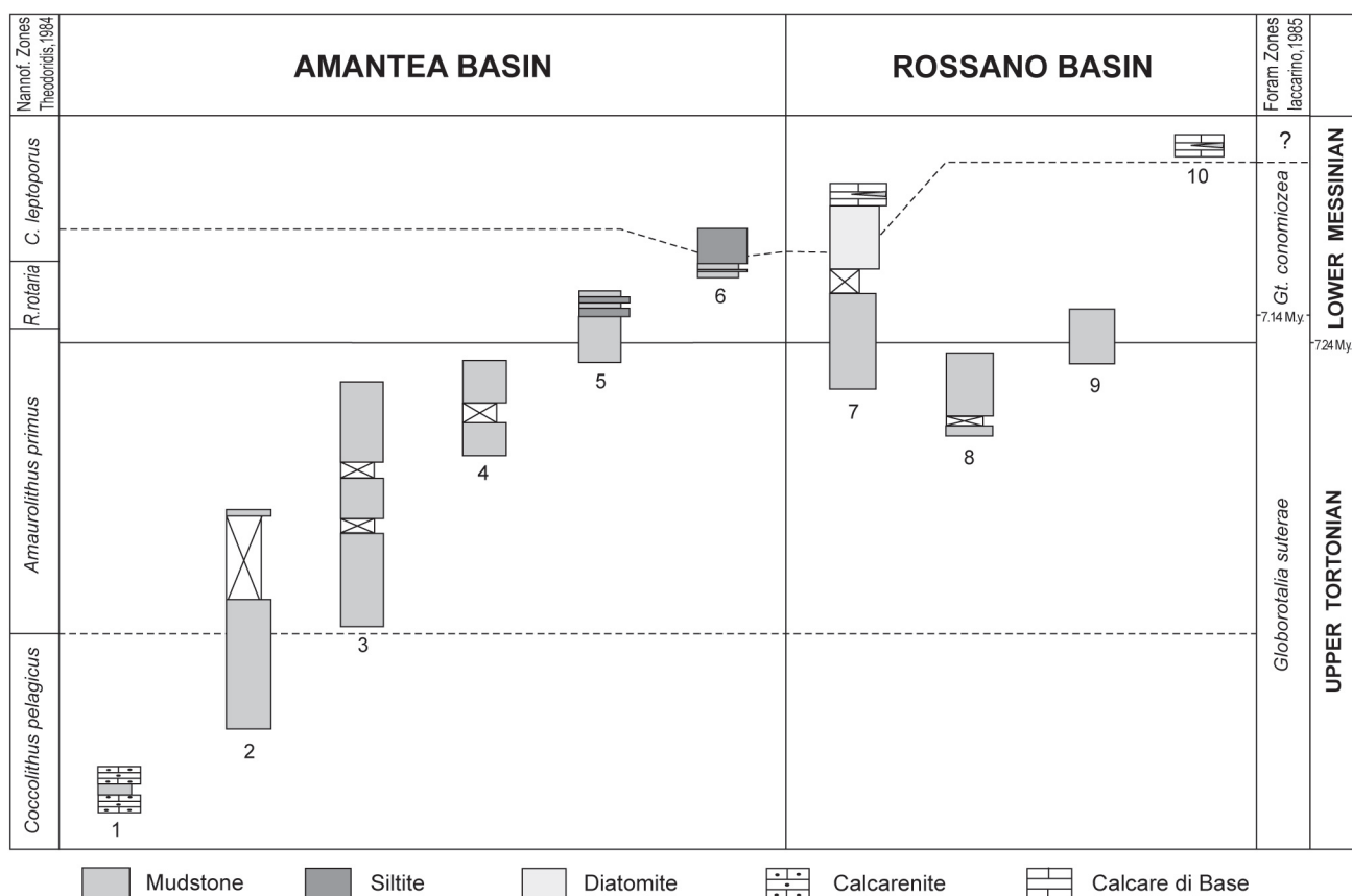
1 = Timpone Napoli section; 2, 3, and 4 = Vallone Salina I, II, and III sections; 5 = Case Vespano section; 6 = Cozzo Salice section; 7 = Vallone Casino section; 8, 9, and 10 = Cozzo Sant'Isidoro I, II, and III sections.
