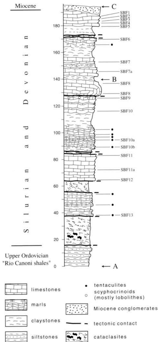
Text-fig. 2 - Lithological column of the SBF Section.
