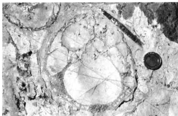
Text fig. 4 - Detail of a slab bearing several crinoid remains, among which well preserved cirrus lobolithes and fragments of stems. Late Silurian, Pridoli, detortus Zone.
