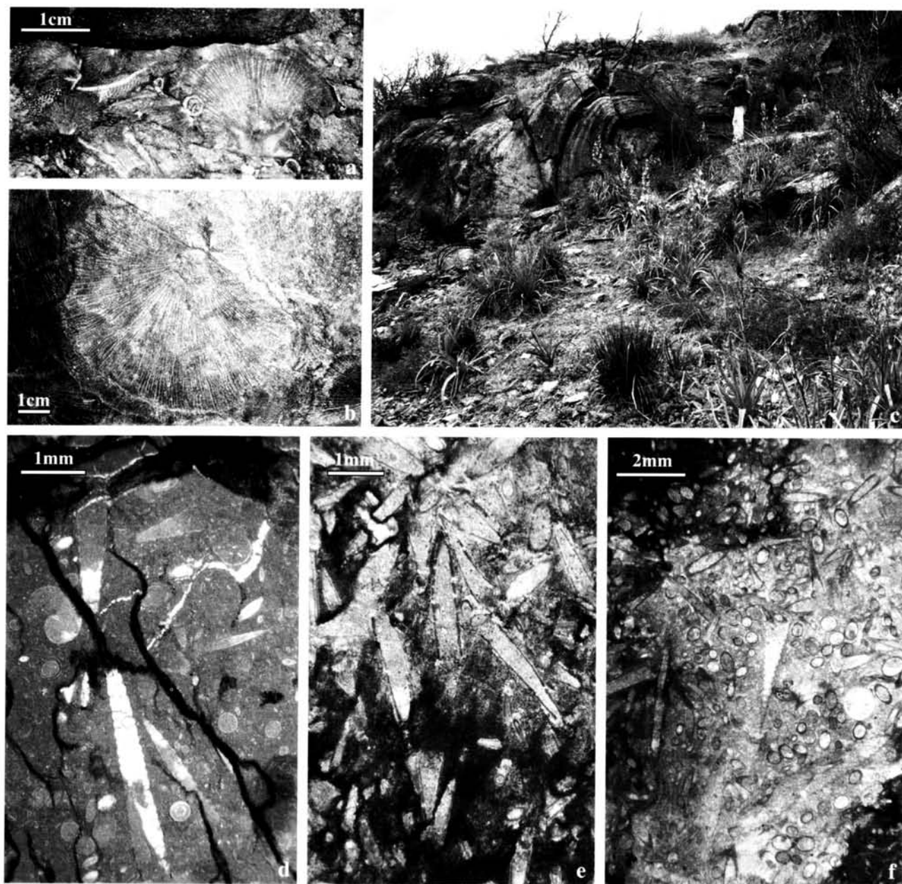
Text-fig. 3 - a) Typical assemblage occurring in the Late Ordovician siltstones of Rio Canoni shales; b) Specimen of Longvillia mediterranea Havlicek from the Rio Canoni shales; c) Overturned anticline in the mid-part of the section (sample SBF 8); d) Dacryoconarids and gastropods microfacies, sample SBF 10b, Lochkovian; e) Dacryoconarids microfacies, sample SBF 13, Frasnian; f) Dacryoconarids microfacies, sample SBF 10a, Emsian.
