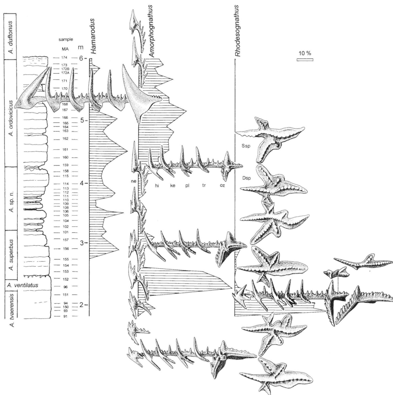
Text-fig. 3 - Changes in relative contribution to samples of the main lineages of conodonts with elaborate apparatuses. Note the restricted occurrences of warm-water Welsh immigrant Rhodesognathus and two peaks in abundance of Amorphognathus .
