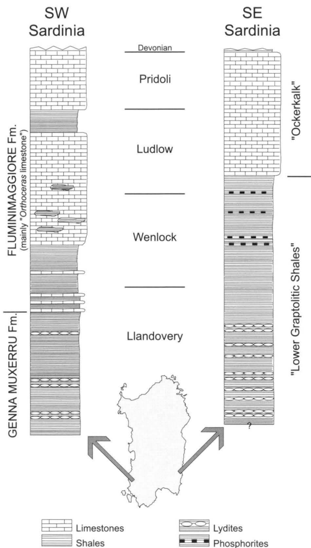
Text-fig. 1 - Sketch stratigraphical columns of the Silurian of Sardinia
