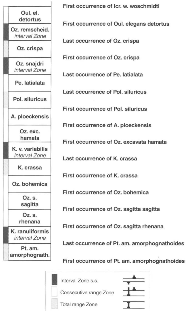
Text-fig. 2 -The Sardinian Silurian Conodont Biozonation
